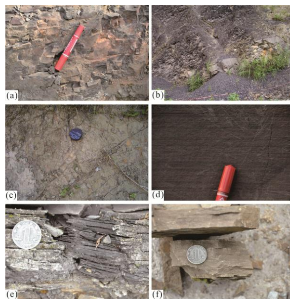
Figure 3. Outcrop characteristics of Wufeng-Longmaxi shale. (a) Black siliceous shale with massive bedding and high hardness; (b) black claystone with laminated bedding; (c) gray siltstone; (d) silty shale with horizontal bedding and cross-layer fractures; (e) black carbonaceous shale with horizontal bedding and low hardness; (f) gray-green muddy siltstone.
